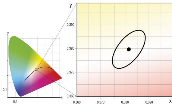
MacAdam ellipse: 3 SDCM
