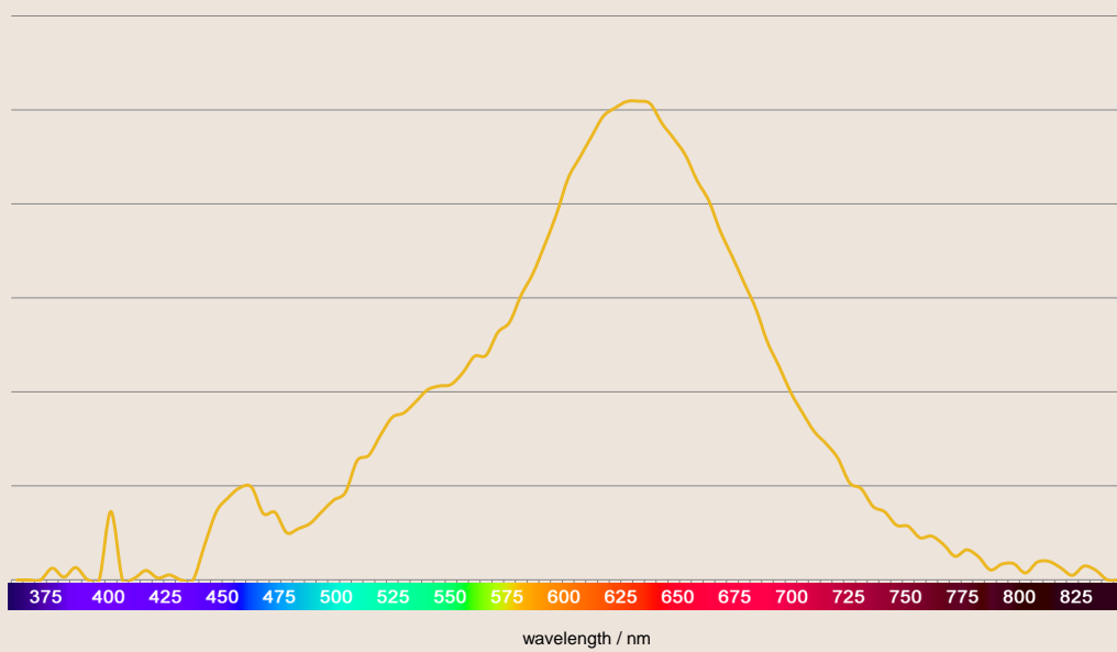
SPECTRAL POWER DISTRIBUTION OF LEDON 1.5W G4
