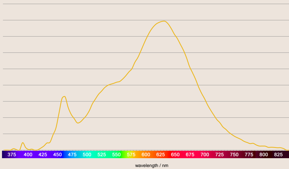
SPECTRAL POWER DISTRIBUTION OF LEDON 5W P45
